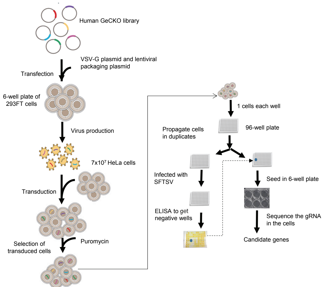
Figure S1. Flow chart of CRISPR-based screen performed in the 96-well plates.
