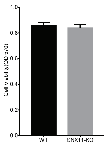
Figure S2. Cell viability assay in the wild-type and SNX11-KO cells.
